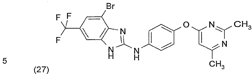
(4-Brom-6-trifluormethyl-1H-benzimidazol-2-yl)-[4-(2,6-dimethyl-pyrimidin-4-yloxy)-phenyl]-amin
